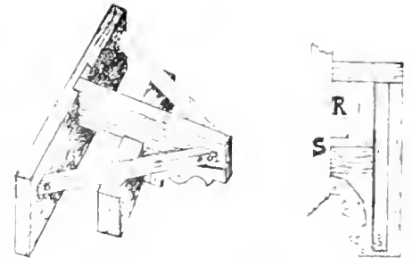
FIG. 1. FIG. 2. No. 121.—TWIN-SLIPPED MOULD.
